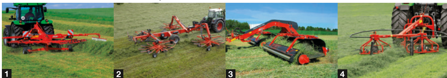
1. Mounted single-rotor rakes 2. Semi-mounted four-rotor rakes 3. Belt mergers 4. Tedder-rake combinations
